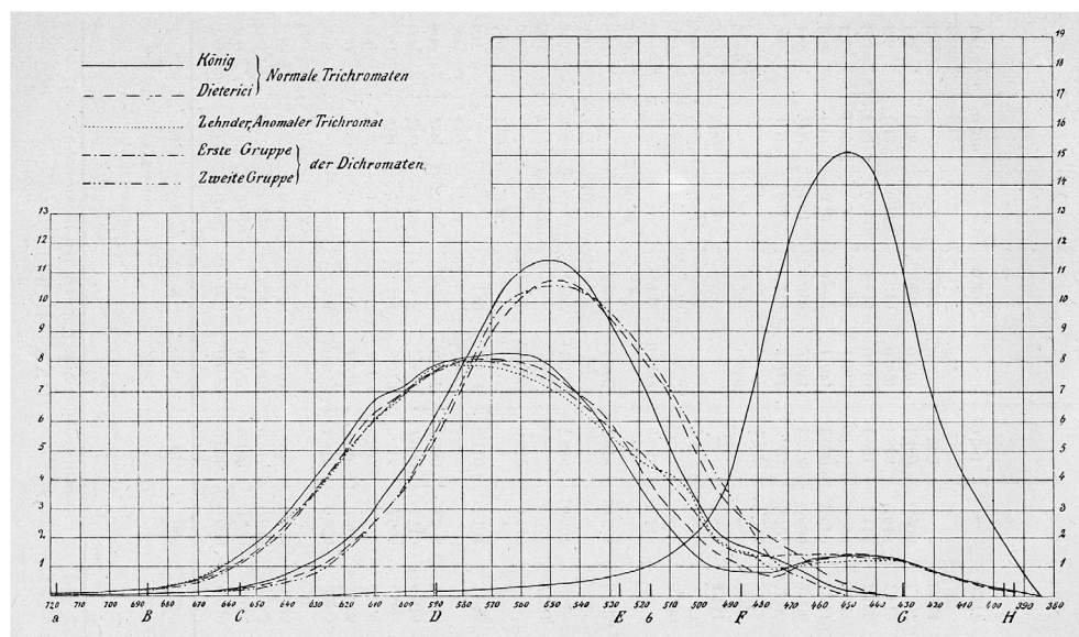
Fig. 1. König's estimates of cone sensitivities (König & Dieterici, 1886). The spectrum is plotted with wavelength decreasing to the right, and the capital letters indicate Fraunhofer lines. The solid lines represent König's own long-wave, middle-wave and short-wave sensitivities and the dashed lines those of his collaborator, Dieterici (whose middle-wave sensitivity differs from König's). Other curves are for anomalous and dichromatic observers.
