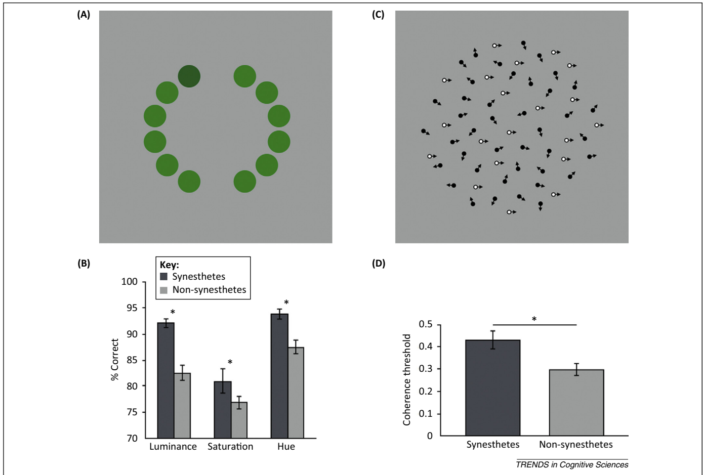
Figure 1. (A) An example of the color visual-search task. (B) Mean accuracy across each color dimension for synesthetes and controls in the visual-search task. The synesthetes performed better than non-synesthetes in all color tasks. (C) A sample random-dot kinematogram display. Dots are randomly positioned within a circular array and move in different directions. The example shown here illustrates 33% coherence: the highlighted dots (33% of the total) all move in the same direction. (D) Mean motion-coherence thresholds for synesthetes and non-synesthetes. The data indicate that synesthetes had reduced motion sensitivity (i.e., higher coherence thresholds) compared with non-synesthetes. (A,B,D) adapted, with permission, from [1].
